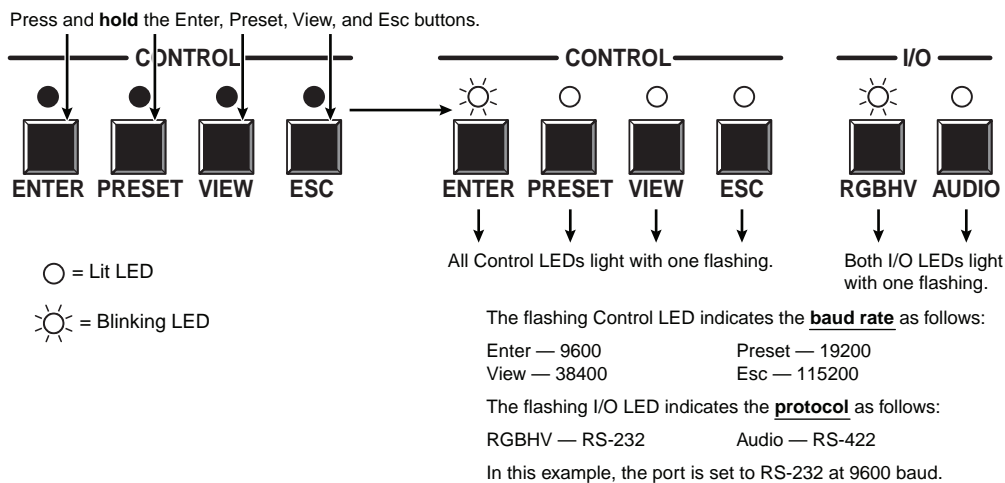
Figure 3-59 — RS-232/RS-422 and baud rate display
