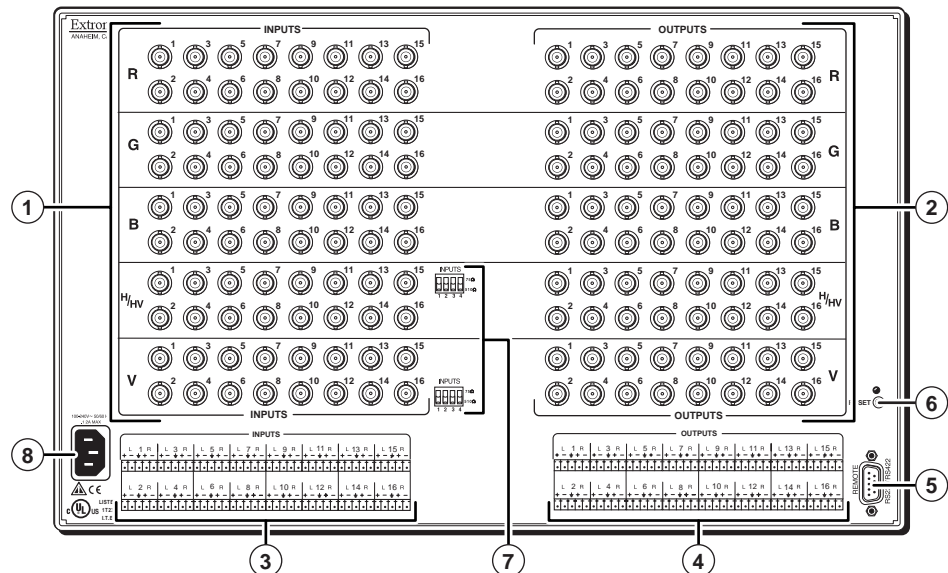
Figure 2-2 — CrossPoint 300 1616 HVA
