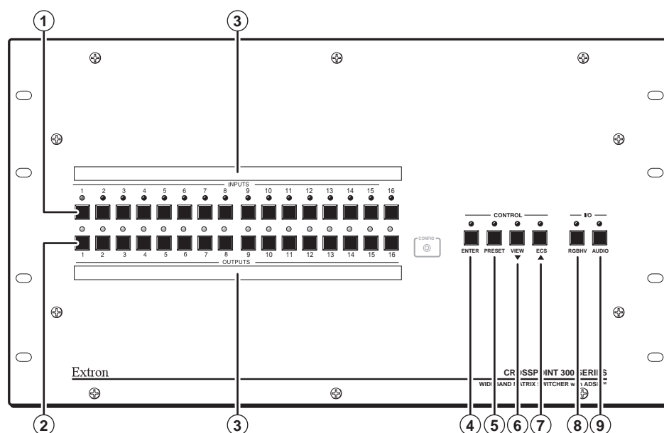
Figure 3-2 — Front Panel, CrossPoint 300 1616 HVA
