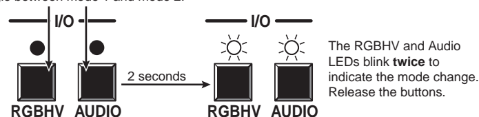
Figure 3-57 — Toggle front panel lock between mode 2 and mode 1
