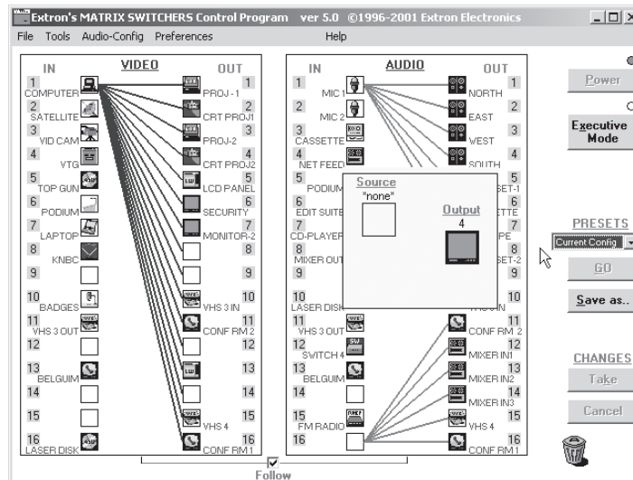
Figure 5-5 — Sample program window (with ties)
