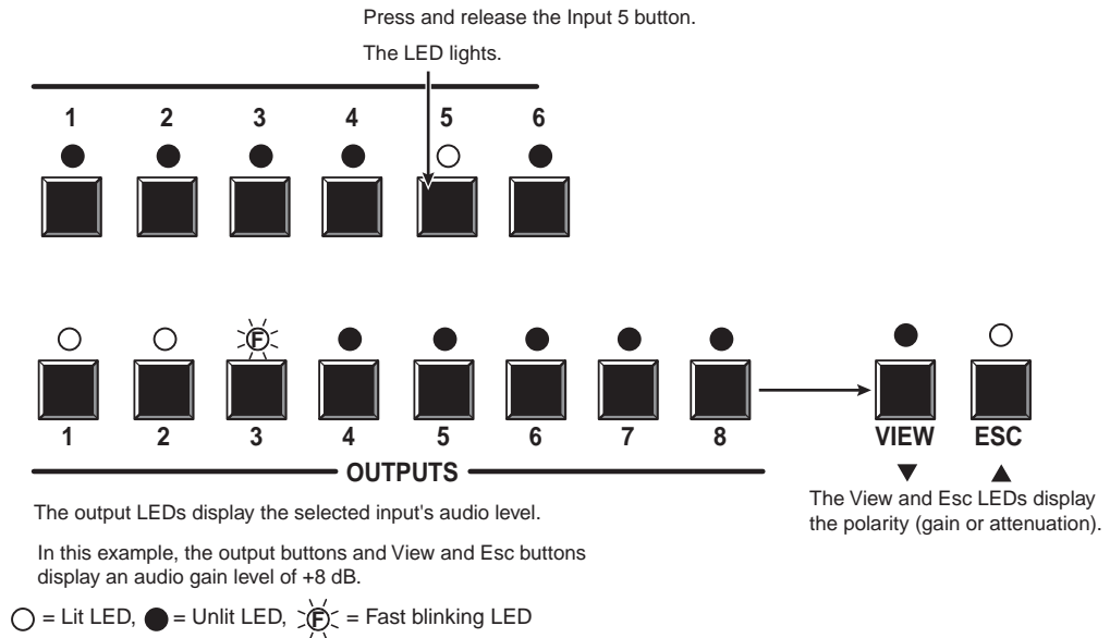
Figure 3-44 — Select an input and level display on an 8-output-LED switcher
