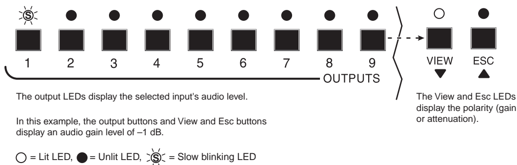
Figure 3-47 — Level display on a 16-output-LED switcher
