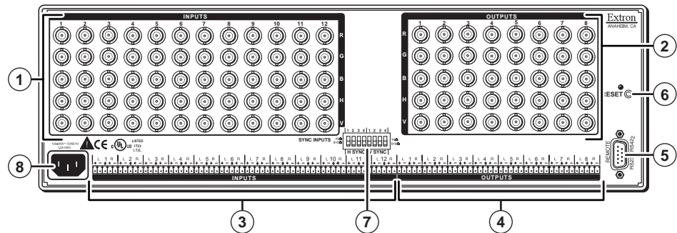
Figure 2-1 — CrossPoint 300 128 HVA
