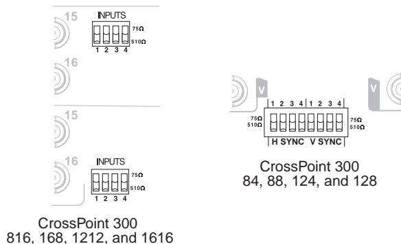
Figure 2-7 — Sync termination switches
