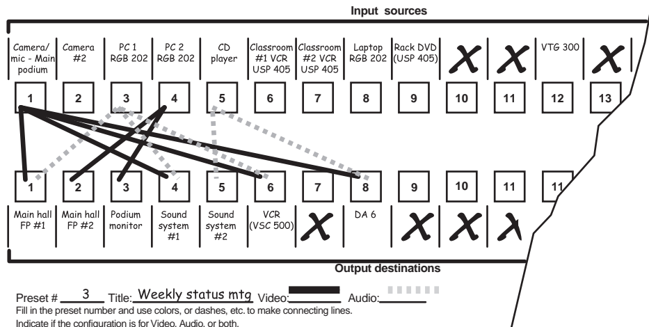
Figure 3-65 — Worksheet example 2: Status meeting configuration
