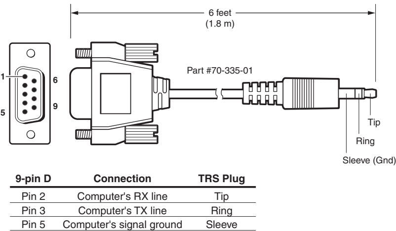
Figure 4-2 — Optional 9-pin TRS RS-232 cable
