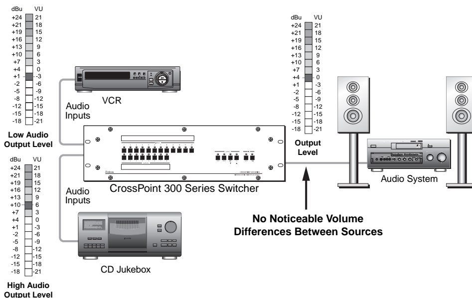
Figure 3-41 — Audio gain and attenuation
