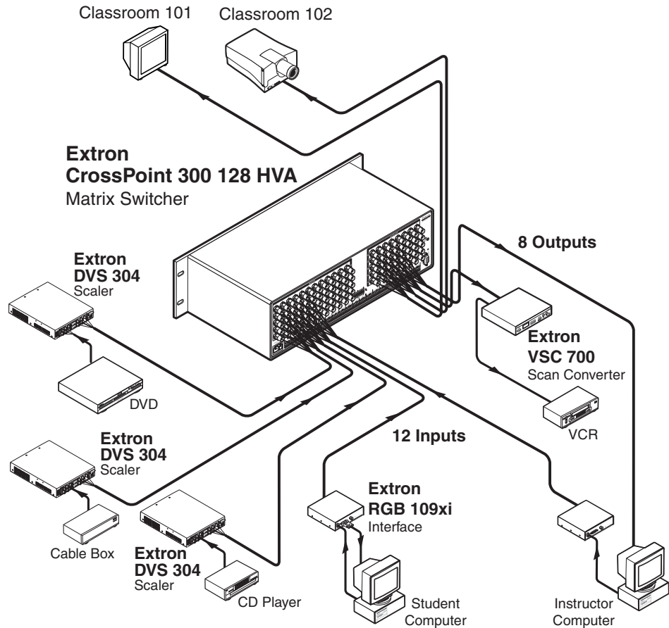
Figure 1-1 — Typical CrossPoint matrix switcher application
