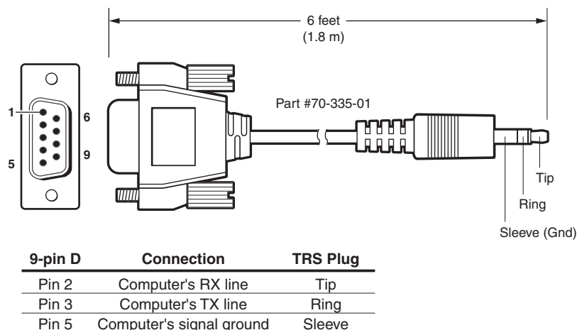
Figure 2-9 — Optional 9-pin TRS RS-232 cable
