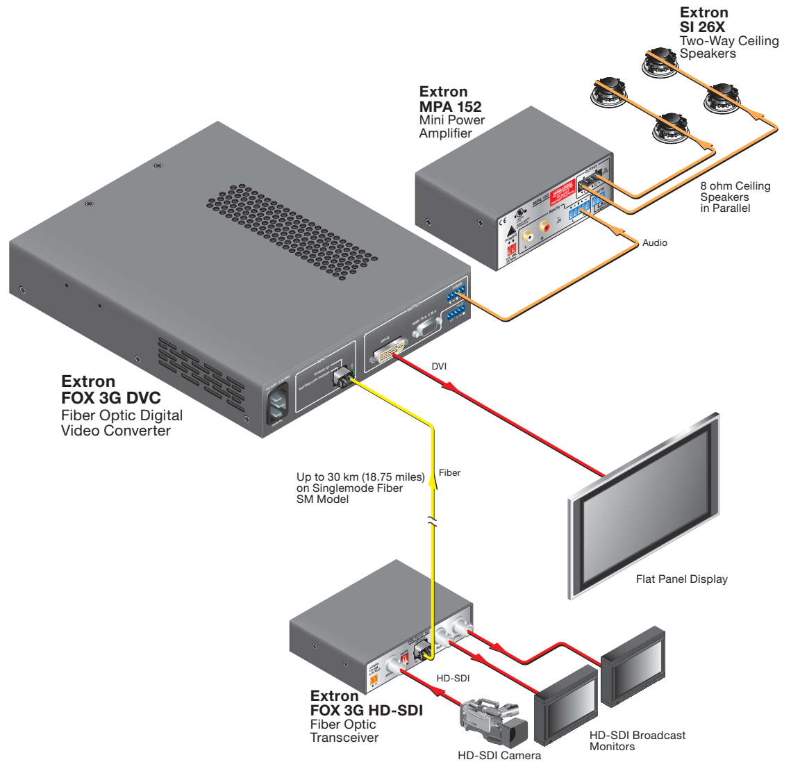
Figure 1. Connection Diagram for a FOX 3G DVC
