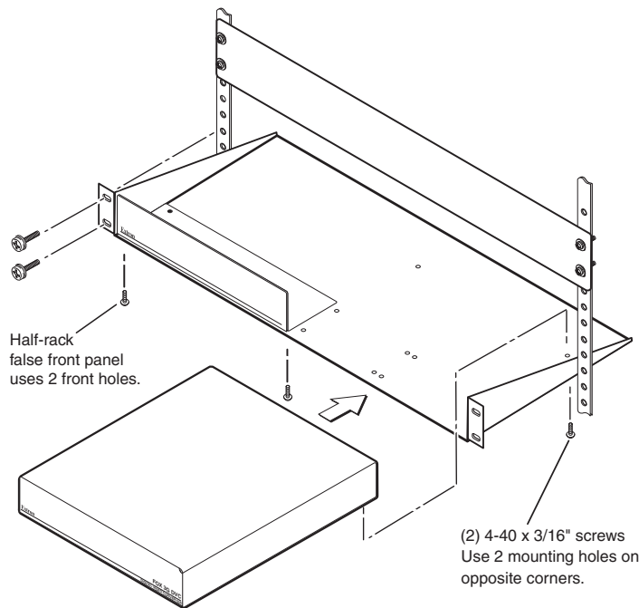
Figure 27. Rack Mounting the FOX 3G DVC
