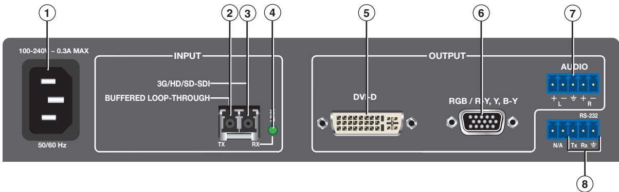
Figure 2. FOX 3G DVC Rear Panel
