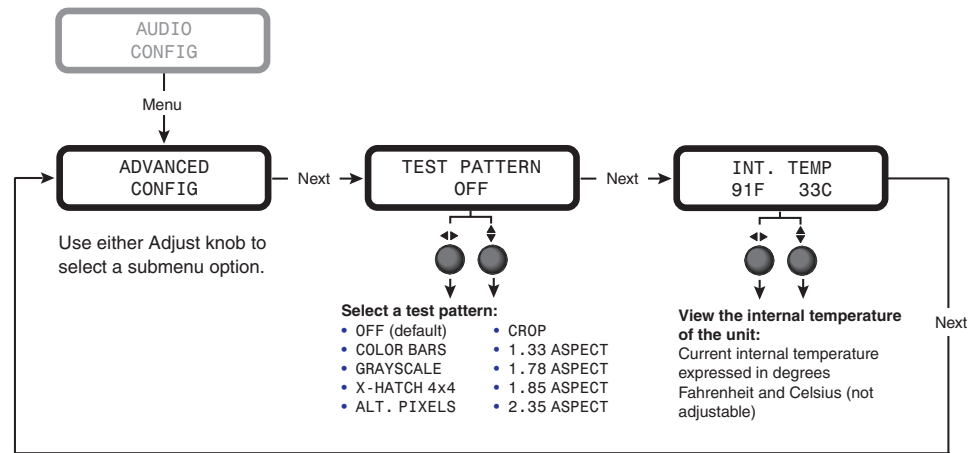
Figure 18. Advanced Config Menu
