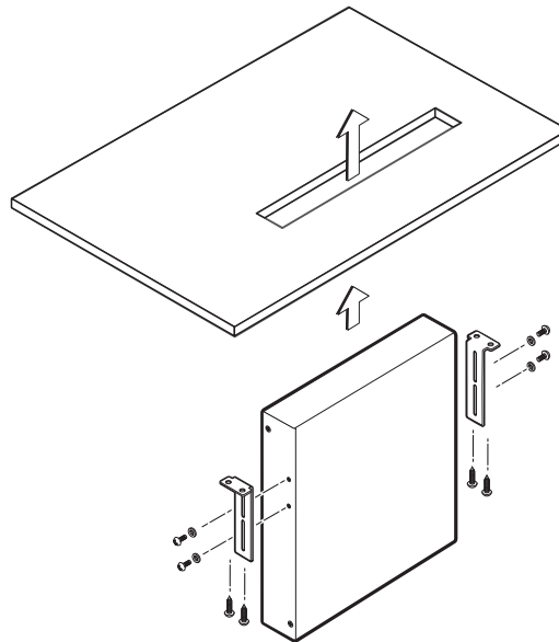
Figure 28. Through-desk Mounting the FOX 3G DVC
