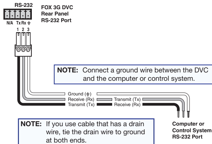
Figure 5. Connecting to the RS-232 Port
