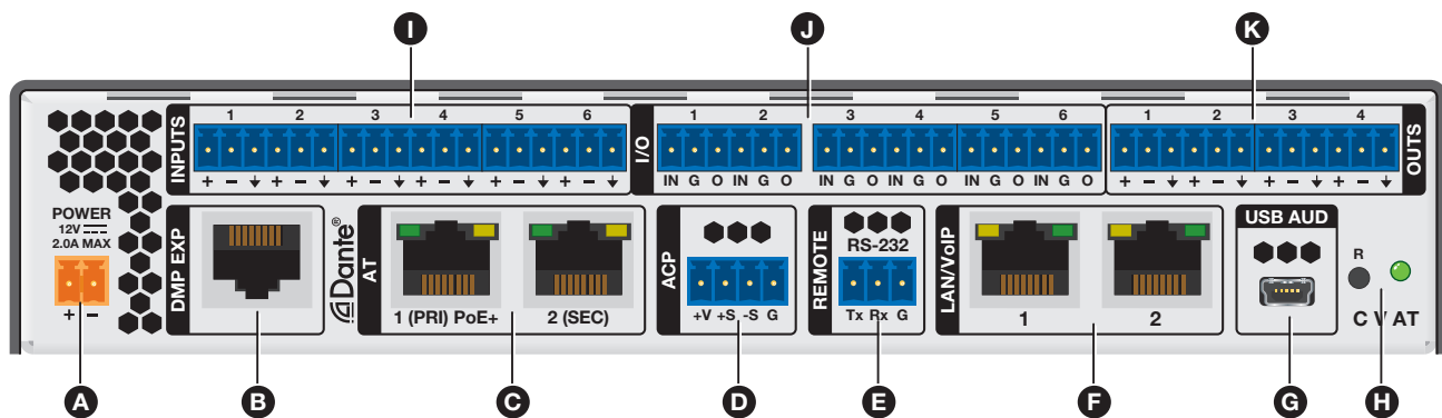
Figure 1. DMP 64 Plus C V AT Rear Panel
