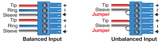
Figure 2. 6-pole Audio Input Wiring
