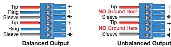
Figure 3. Audio Output Wiring
