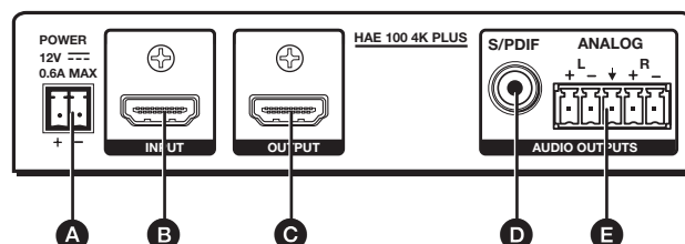
Figure 3. HAE 100 4K Plus Rear Panel
