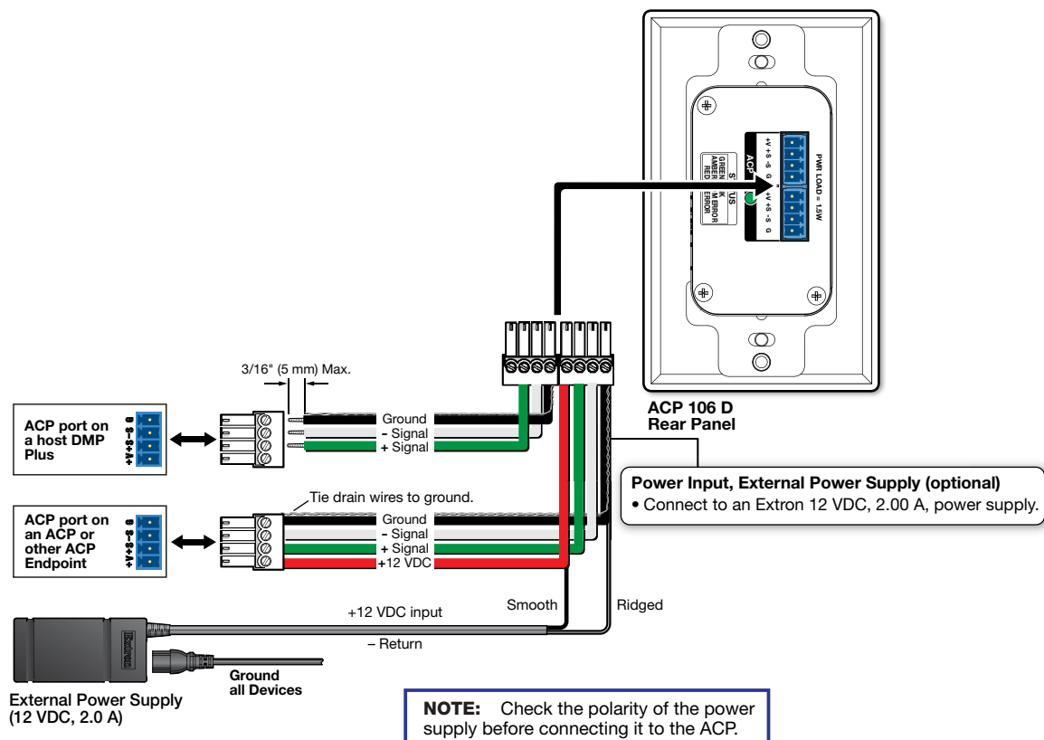
Figure 5. Cabling ACP Panels with an Extron 12 VDC Power Supply
