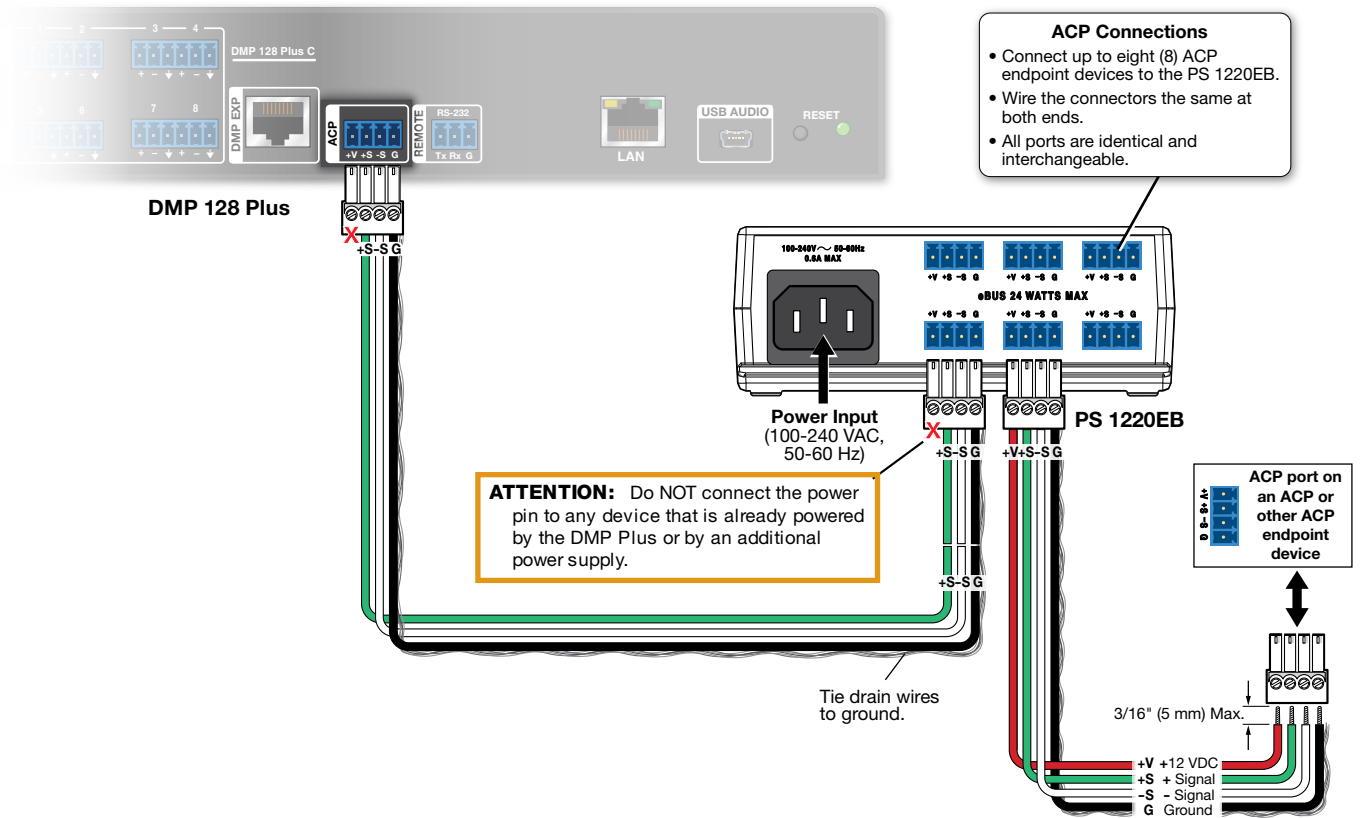
Figure 4. Cabling ACP Devices with a PS 1220EB Power Inserter
