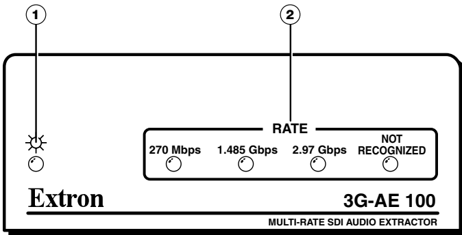
Figure 2. 3G-AE 100 Front Panel
