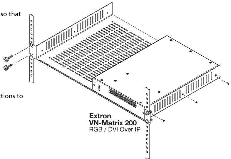
Figure 1. Installation of a Unit to the Dual Rack Mounting Kit
