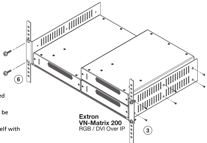
Figure 2. Installation of a Unit to the Quad Rack Mounting Kit
