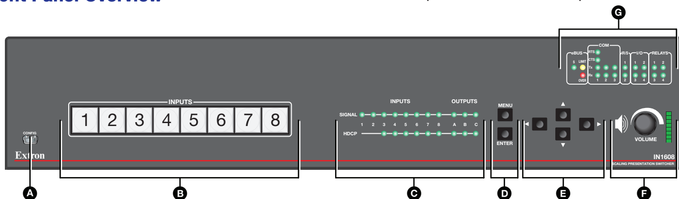
Figure 2. Front Panel Features (IN1608 IPCP SA HDBT Shown)
