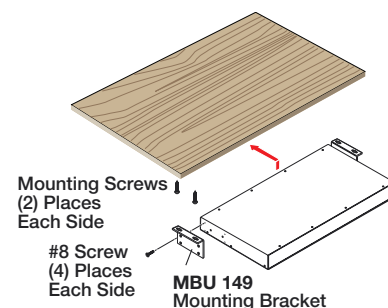
Furniture Mounting
