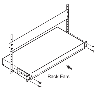
Rack Mounting
