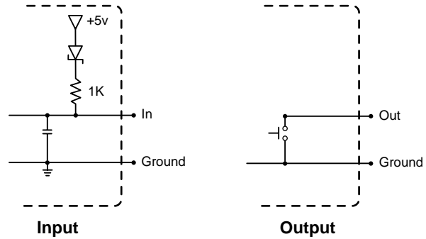
Figure 3. CCR AAP Input and Output Schematics
