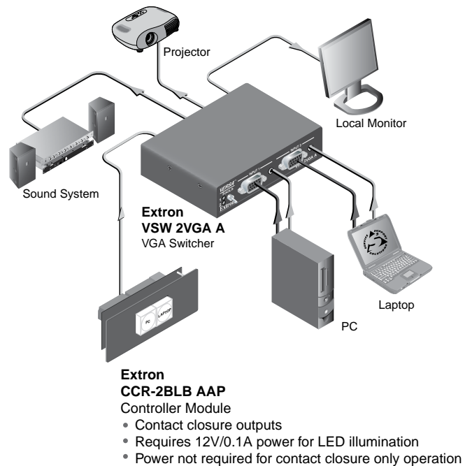
Figure 5. Typical CCR-2BLB AAP Application
