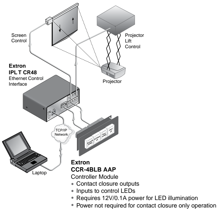
Figure 4. Typical CCR-4BLB AAP Application
