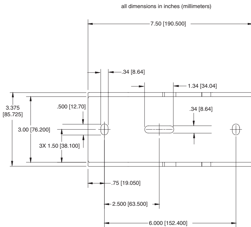
Figure 3. ACMP 100 Dimensions
