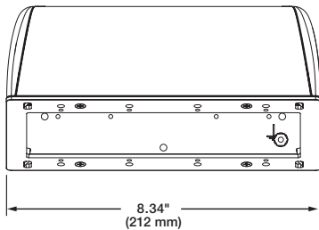
Top View - 4 Gang
