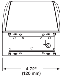
Top View - 2 Gang
