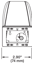
Top View - 1 Gang
