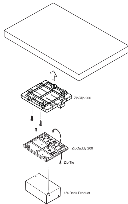
ZipClip 200 under-desk mounting of quarter-rack width enclosure
