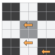
Nearest Neighbor
