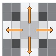
Bilinear Interpolation
