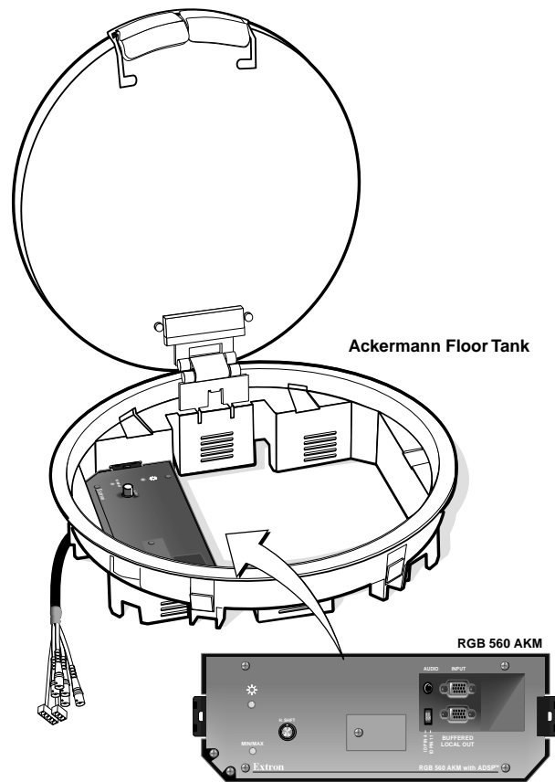
Figure 1 — Interface components
