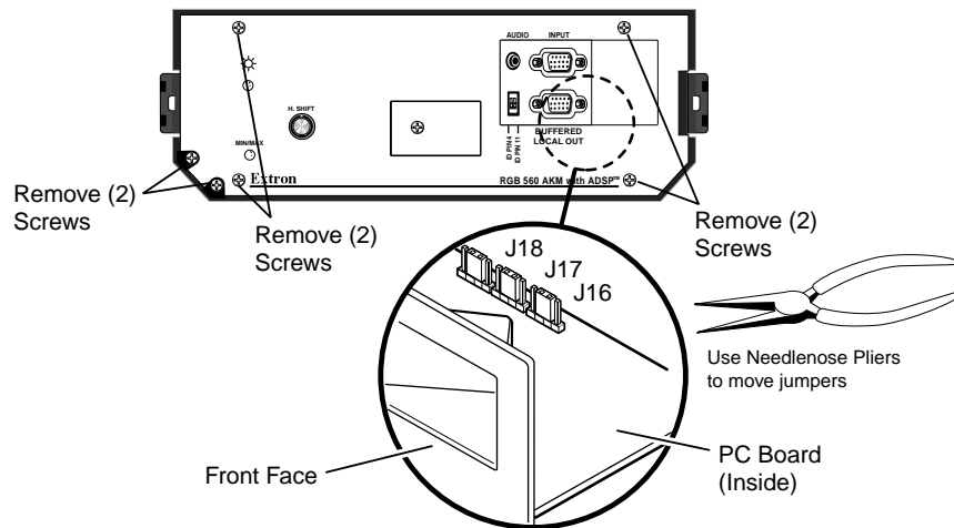
Figure 4 — Setting the gain/peaking jumpers
